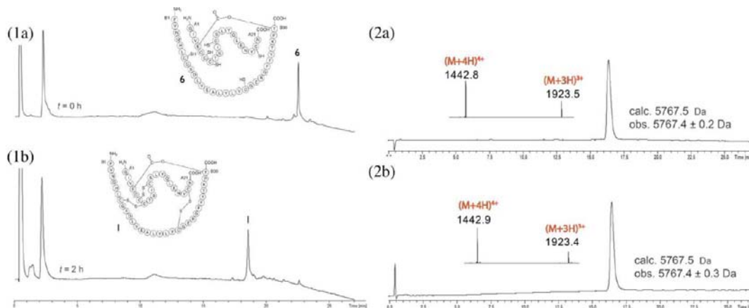
Figure 2. Folding of ester insulin. Folding was carried at room temperature in a pH 7.6 buffer solution containing 1.5 M GnHCl, 20 mM Tris, 8 mM cysteine, 1 mM cystine·HCl, at a starting polypeptide concentration of ~0.3 mg/mL. (1a) Crude linear polypeptide ester insulin (6) at t = 0 h. (1b) Folding reaction after 2 h. The chromatographic separations were performed on a C18 column using a linear gradient (4–48%) of buffer B in buffer A over 22 min (buffer A = 0.1% TFA in water, buffer B = 0.08% TFA in acetonitrile). (2a) Folded L-ester insulin after prep HPLC purification (Inset: online ESI-MS spectra of the main peak). (2b) Folded D-ester insulin after prep HPLC purification (Inset: online ESI-MS spectra of the main peak). The chromatographic separations were performed on a C18 column using a linear gradient (9%–53%) of buffer B in buffer A over 22 min.
