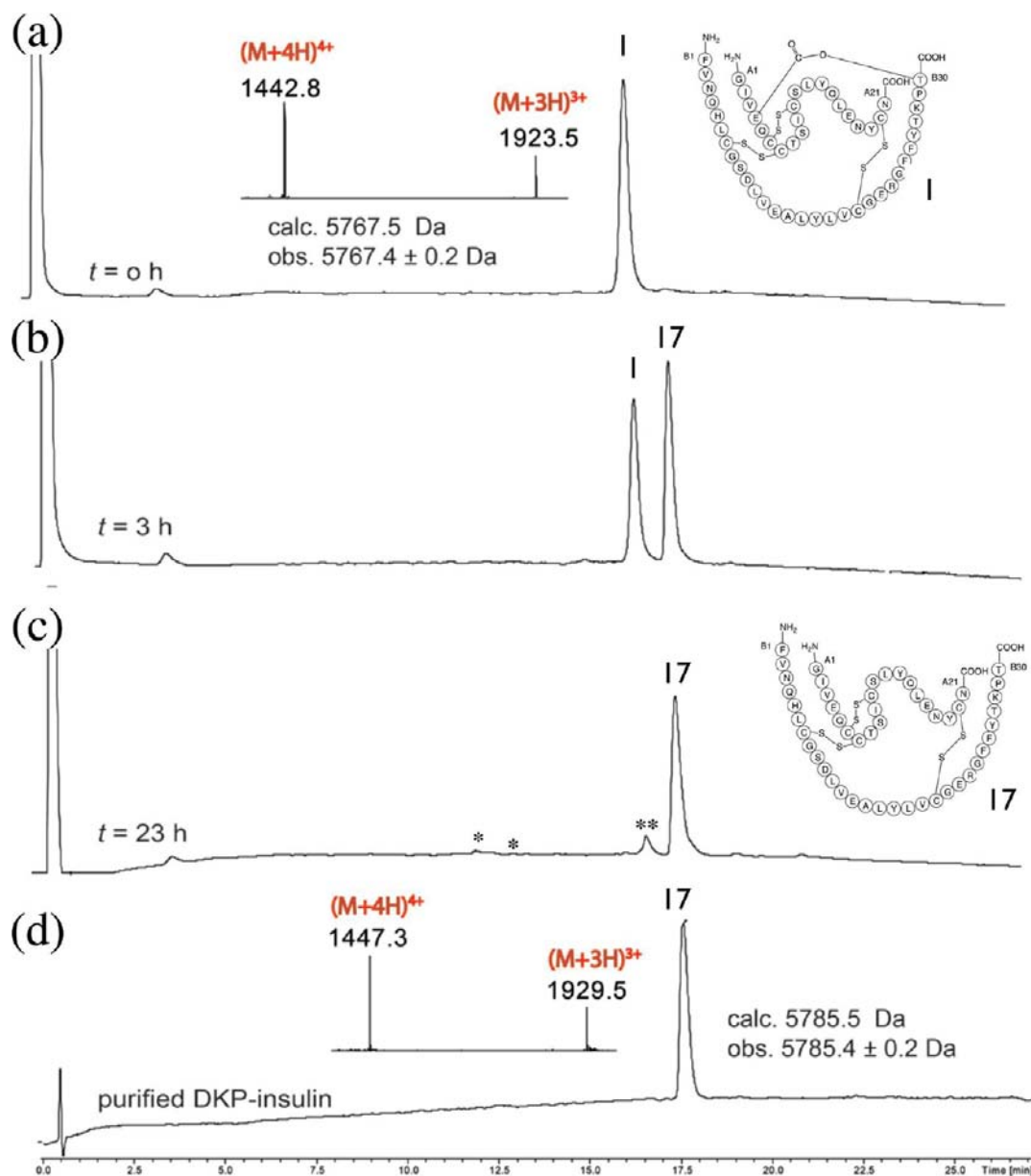
Figure 4. Conversion of DKP ester insulin to native DKP insulin. Saponification of ester insulin 1 to give DKP insulin 17 : (a) Ester insulin 1 at t = 0 h (Inset: online ESI-MS spectra of the main peak). (b,c) Reaction mixture at (b) t = 3 h and (c) t = 23 h. *: derived from A chain. **: oxidized B chain. (d) Purified DKP insulin (Inset: online ESI-MS spectra of the main peak). The observed increase of 18 Da for the hydrolyzed DKP insulin confirms the conversion of ester insulin into DKP insulin by addition of the elements of water. The chromatographic separations were performed on a C18 column using a linear gradient (9–53%) of buffer B in buffer A over 22 min.
