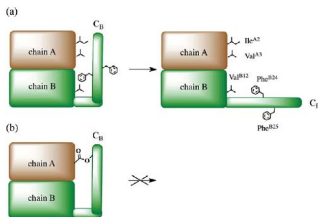
Figure 6. Conformation affects insulin binding to its receptor. (a) Schematic illustration of conformational change of insulin upon its binding to the receptor, after Weiss et al. 49 Chains A and B are schematically shown as brown and green regions, respectively. Residues Ile A2 , Val A3 , Val B12 , Phe B24 , and Phe B25 implicated in binding to the insulin receptor are schematically shown. (b) Schematic model of ester insulin 'locked' in an unproductive conformation by the ester tether.
