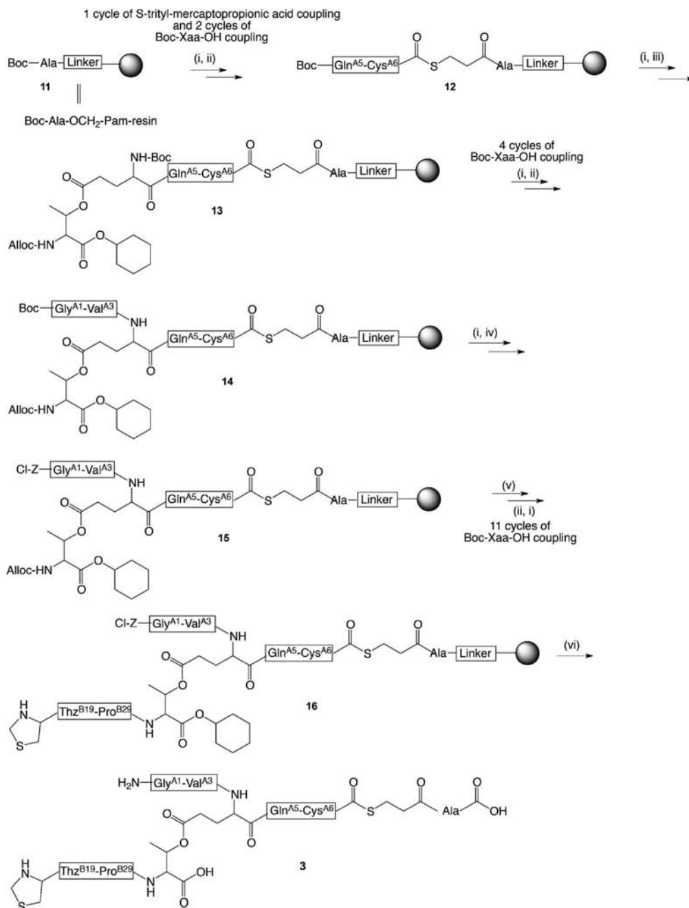
Scheme 3. Solid Phase Synthesis of Thz B19 -[Al 1 -Glu A4 (O \beta Thr B30 )-Al 6 - \alpha COS A
