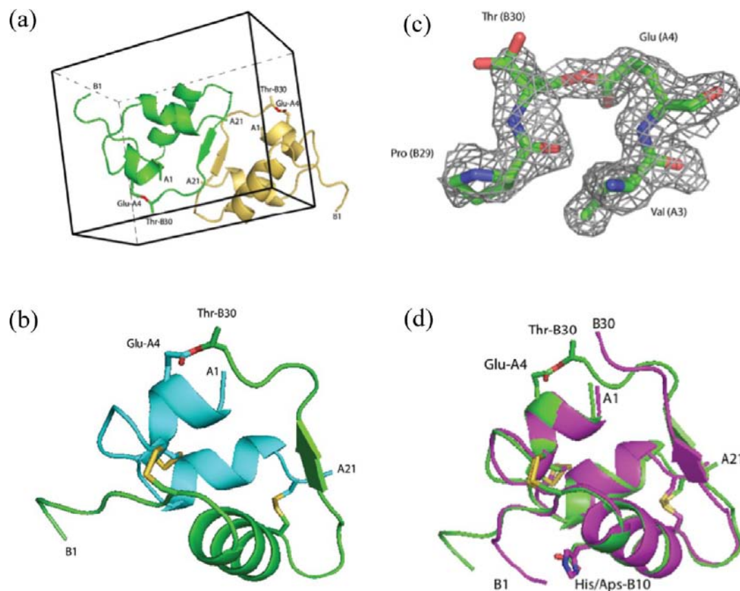
Figure 3. X-ray structure of ester insulin (1.6 Å), obtained from racemic crystallization of D-DKP ester insulin and L-DKP ester insulin. (a) Racemic crystal packing in centrosymmetric P\bar{1} unit cell, showing the L-DKP ester insulin molecule (green) and the D-DKP ester insulin molecule (gold). The ester linkage is shown in sticks (O, red). (b) Cartoon representation of the A chain (cyan) and B chain (green) of L-DKP ester insulin. The three disulfide bonds of the folded protein and the ester linkage are shown as sticks (O, red; S, gold). (c) SigmaA-weighted 2Fo-Fc electron density map, contoured at 1.5\sigma , showing the ester linkage between Glu A4 -Thr B30 (C, green; O, red; N, blue). (d) Superposition of X-ray crystal structures of the T-form of KP insulin (PDB ID: 1LPH) (magenta) and DKP ester insulin (green). The three disulfide bonds and the ester linkage are shown as sticks (O, red; N, blue S, gold).
