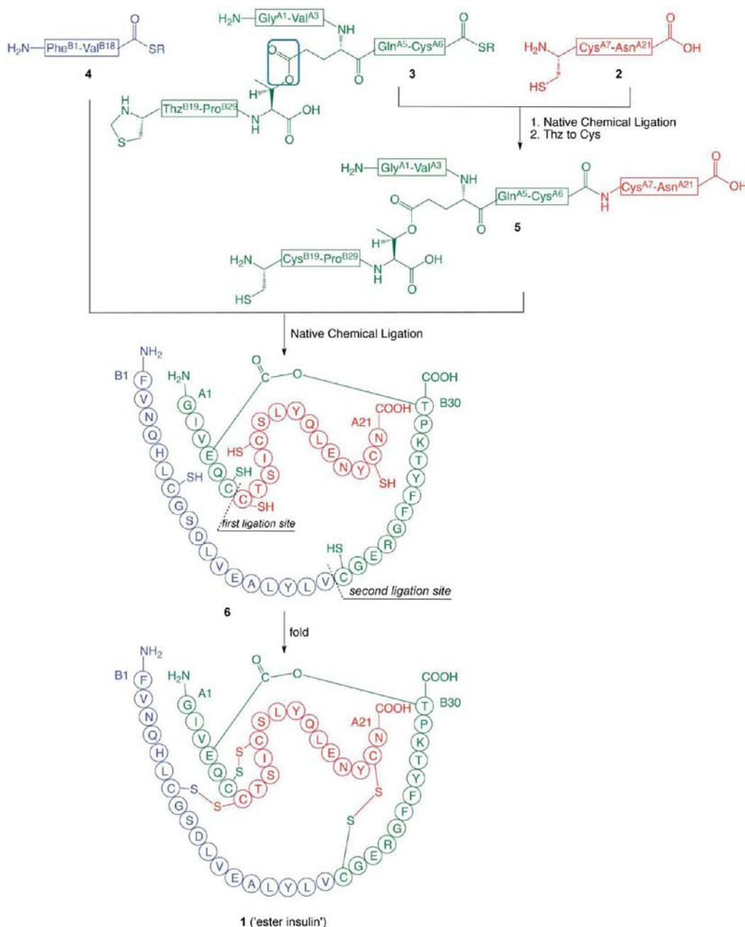
Scheme 1. Convergent Synthetic Strategy from Three Peptide Segments of Approximately Equal Size Used for the Total Chemical Synthesis of DKP Ester Insulin by “One Pot” Native Chemical Ligations ( R = -CH_2CH_2CO-Ala-COOH ) a
