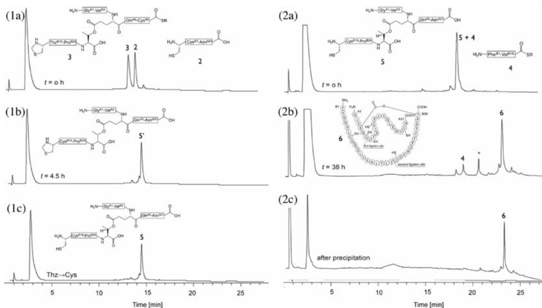
Figure 1. One pot reactions for the total chemical synthesis of the ester insulin polypeptide 6. (1) Native chemical ligation for the synthesis of Gly A1 -Glu A4 [OβThr B30 -Cys B19 ]-Asn A21 (5). (1a-b) Reaction of peptide segments Gly A1 -Glu A4 [OβThr B30 -Thz B19 ]-Cys A6 .αCOSR (3) (R = -CH 2 CH 2 CO-Ala-COOH) and Cys A7 -Asn A21 (2). (1c) Conversion of Thz- to Cys-. The chromatographic separations were performed on a C18 column using a linear gradient (9%–53%) of buffer B in buffer A over 22 min (buffer A = 0.1% TFA in water, buffer B = 0.08% TFA in acetonitrile). (2) Native chemical ligation for the synthesis of Gly A1 -Glu A4 [OβThr B30 -Phe B1 ]-Asn A21 (6). (2a-b) Reaction of Gly A1 -Glu A4 [OβThr B30 -Cys B19 ]-Asn A21 (5) and Phe B1 -Val B18 .αCOSR (4). Both peptide segments have the same retention time, as confirmed by LC-MS. Upon completion, excess Phe B1 -Val B18 .αCOSR (4) remained. *: Phe B1 -Val B18 .αCO-MPAA thioester. (2c) Crude polypeptide (6) after precipitation from water. The chromatographic separations were performed on a C18 column using a linear gradient (4%–48%) of buffer B in buffer A over 22 min. All analyses were by LC-MS; only the HPLC data are shown.
